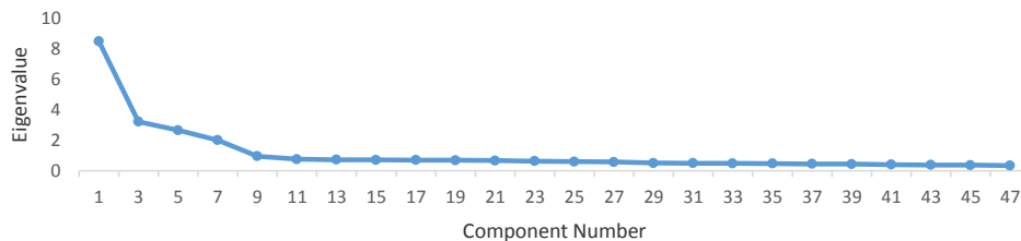
Scree Plot
